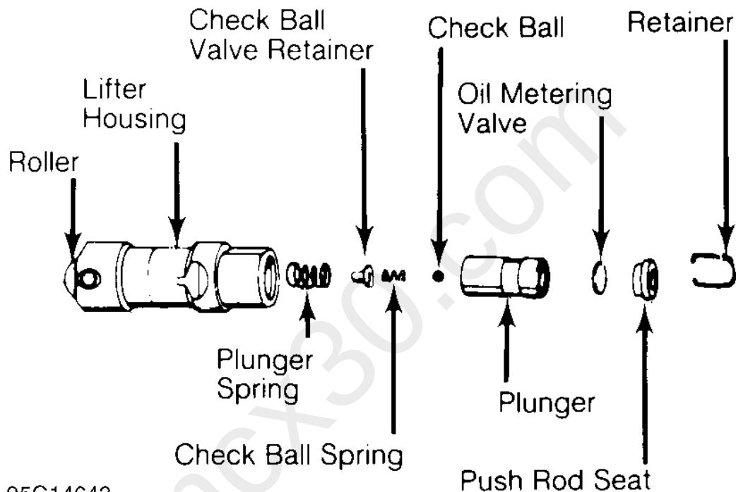
ROLLER LIFTER
